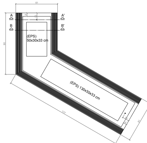
VISTA INFERIOR / BOTTOM VIEW
